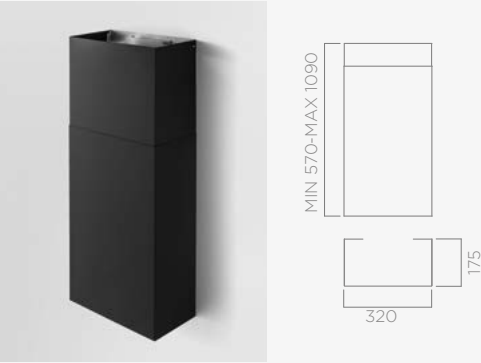
BLACK CHIMNEY KIT
