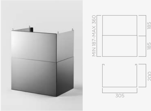
STAINLESS STEEL CHIMNEY KIT H185+H185
